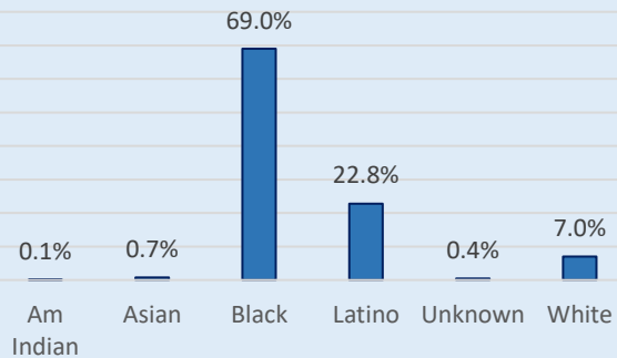
Race Distribution
